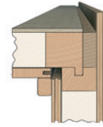
3. Wall to ceiling connection with deep-groove joint.
